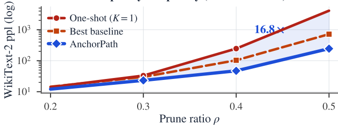
Perplexity vs. sparsity (LLaMA-3.1-8B)
